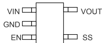
TOP VIEW SOT-23-5
