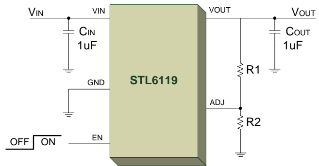
Adjustable Type
