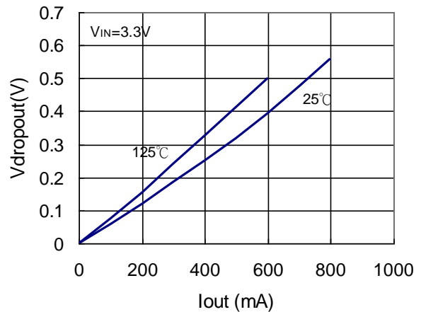
Dropout Voltage
