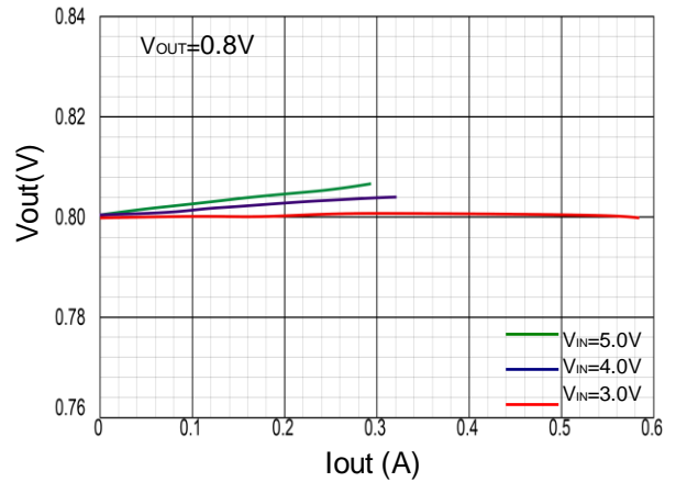
Load Regulation
