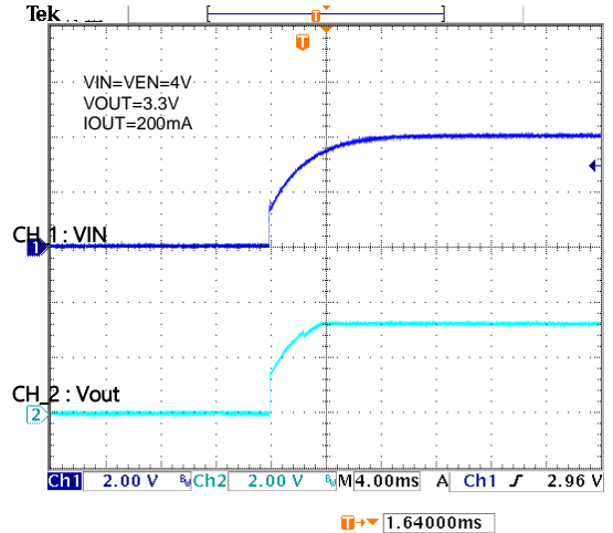
Start-up Waveform
