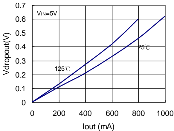
Dropout Voltage
