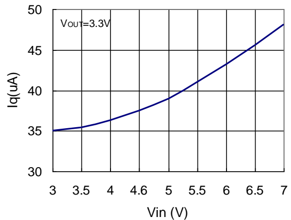
Quiescent current
